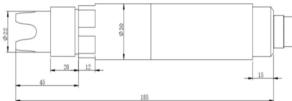
pH Sensor
