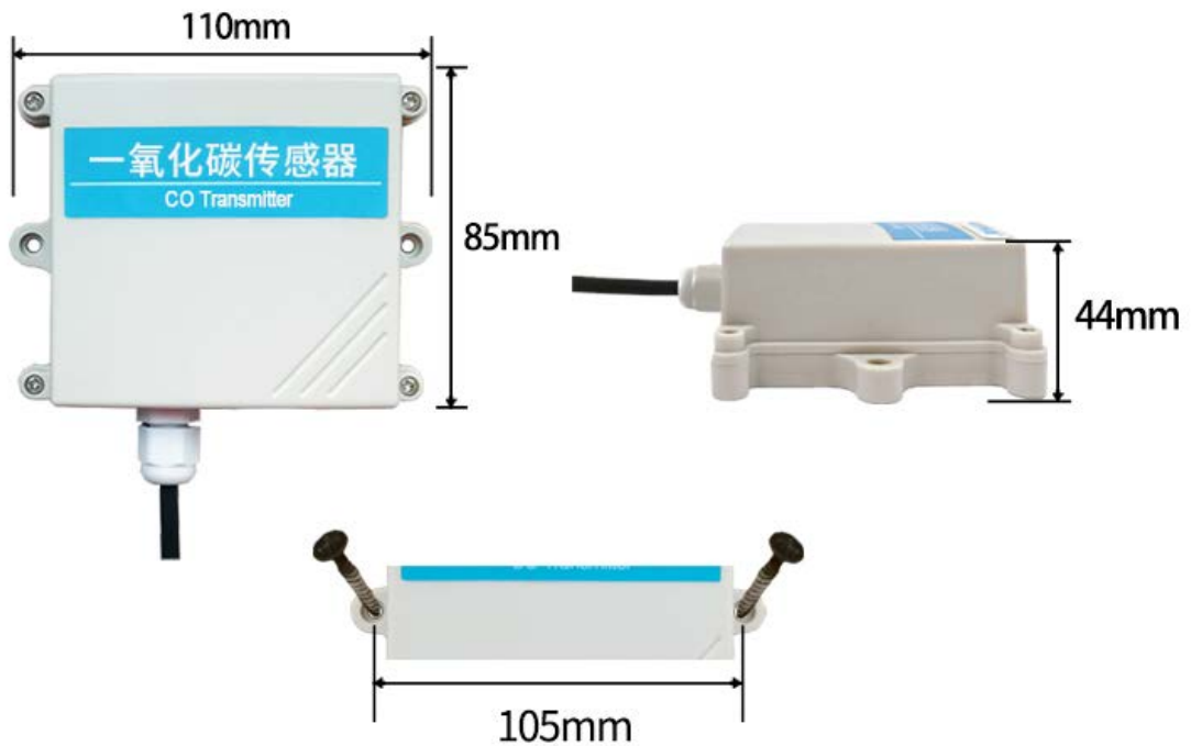
CO Sensor
