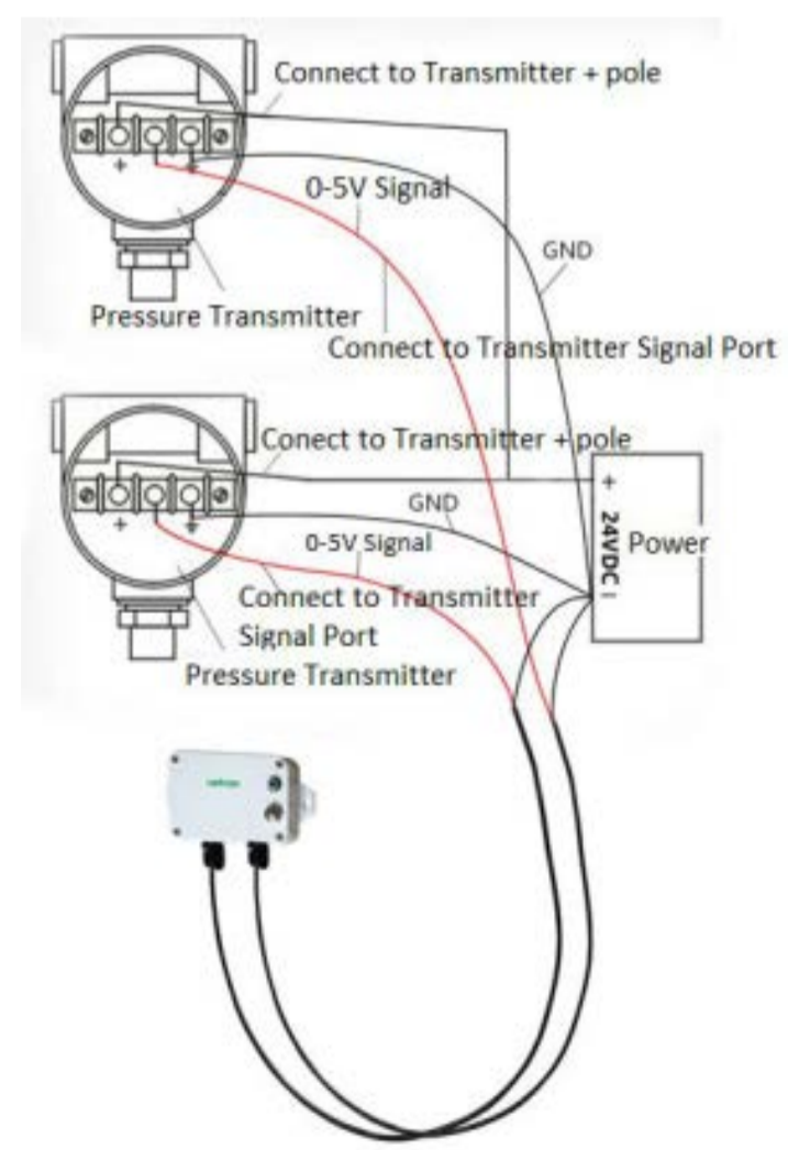
Fig. 3-wire System Example Diagram (for wiring reference)
