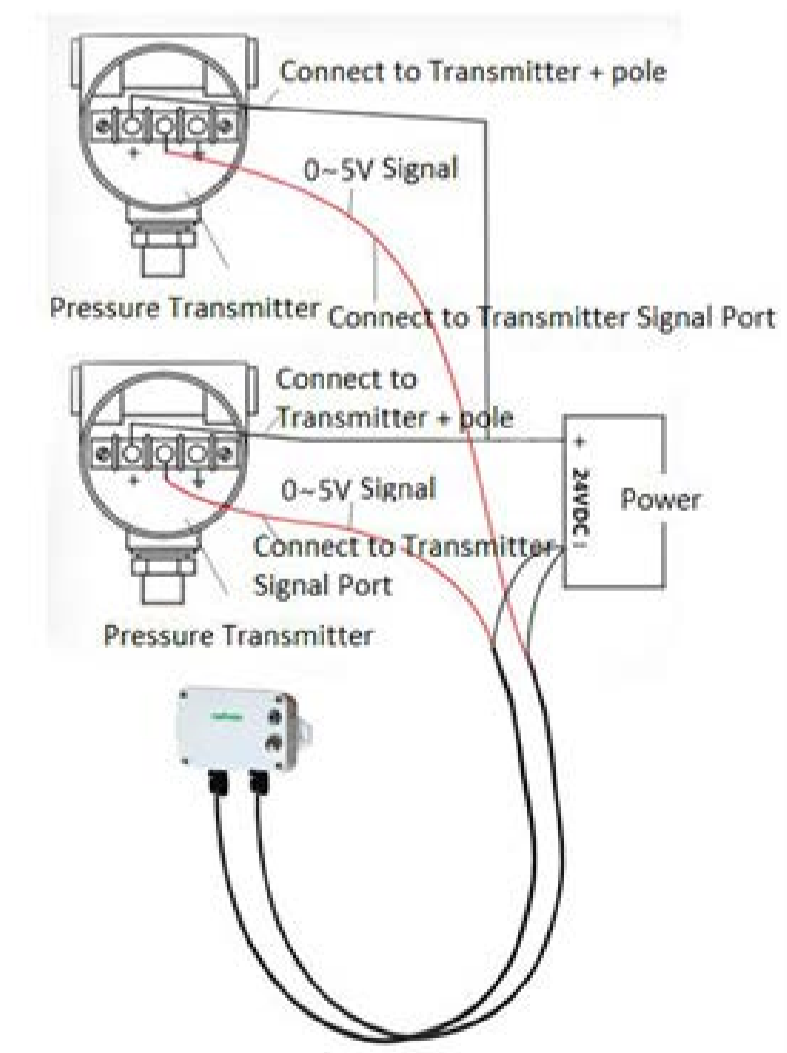
Fig. 2-wire System Example Diagram (for wiring reference)
